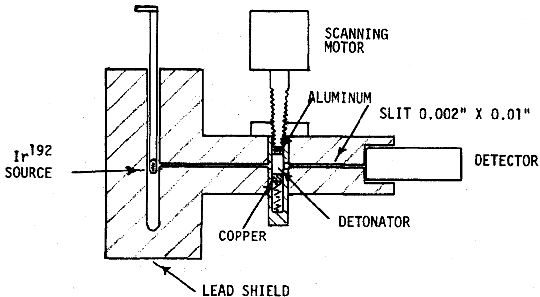
Fig 6 Sketch of \gamma -Ray Density Scanner
